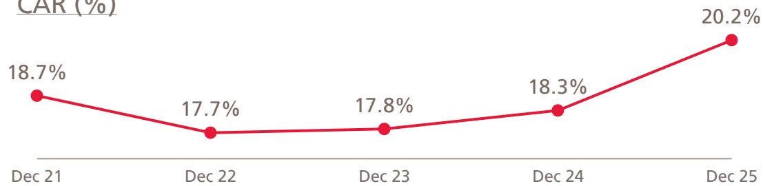
CAR (%)
